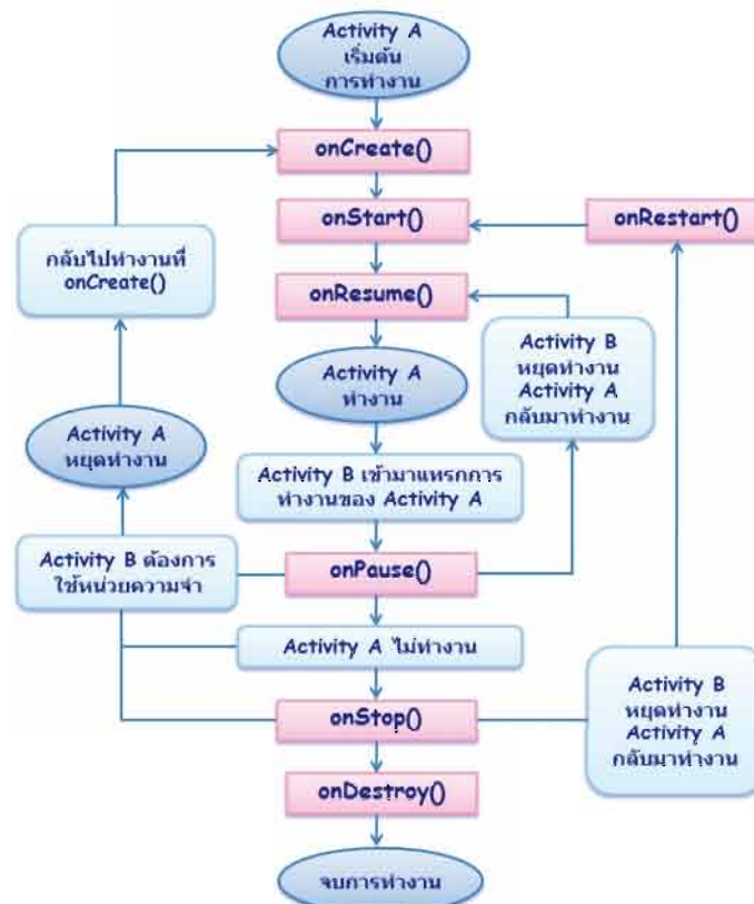
▲ Activity Life Cycle
